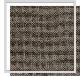
V3/fungi
